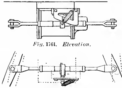
THE HINCKLEY BRAKE SLACK ADJUSTER EQUIPMENT C.
